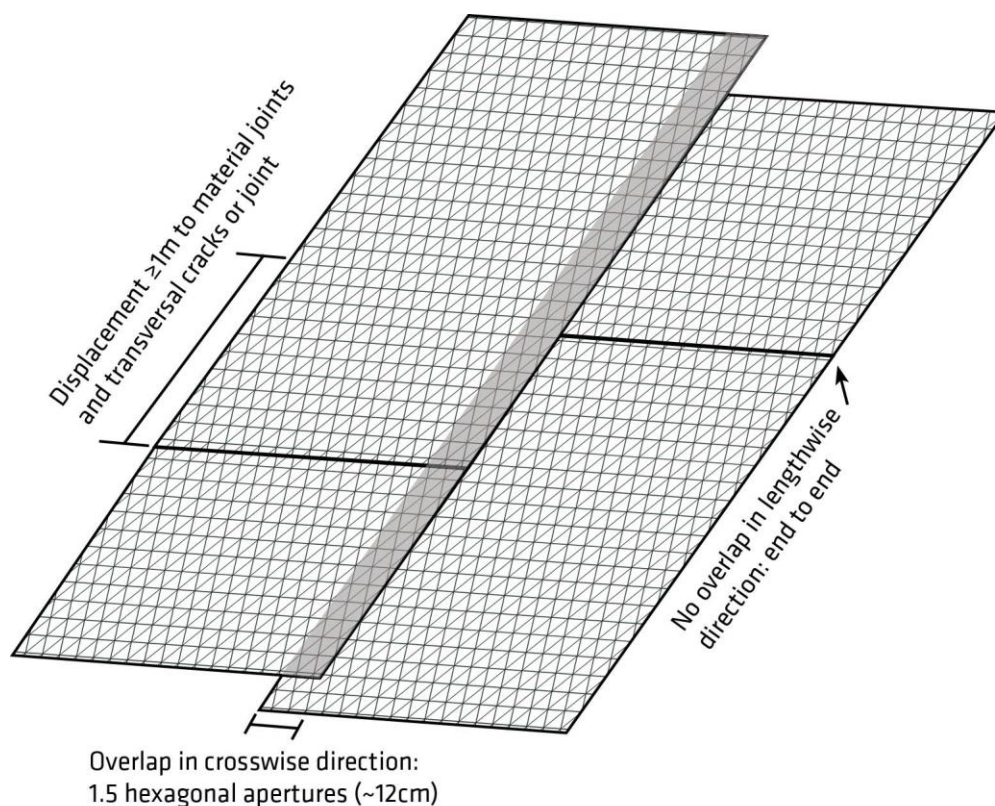
Figure 6: Overlap detail
